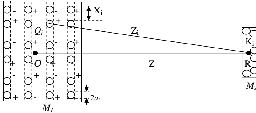
Figure 7.2. A body of mass M_1 containing N_1 positive and negative charges each of magnitude Q_i at a distance Z_i from a point R with mass M_2 in space. Two constituent charges, each of radius a_i , making a pair of particles, are separated by a distance X_i , much larger than a_i . The distance Z_i is much larger than X_i .
