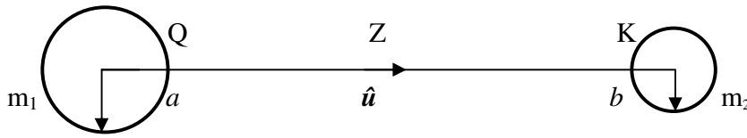
Figure 7.1. Electrostatic and gravitational forces between two charges Q and K .
